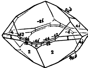
Bergen Hill.
